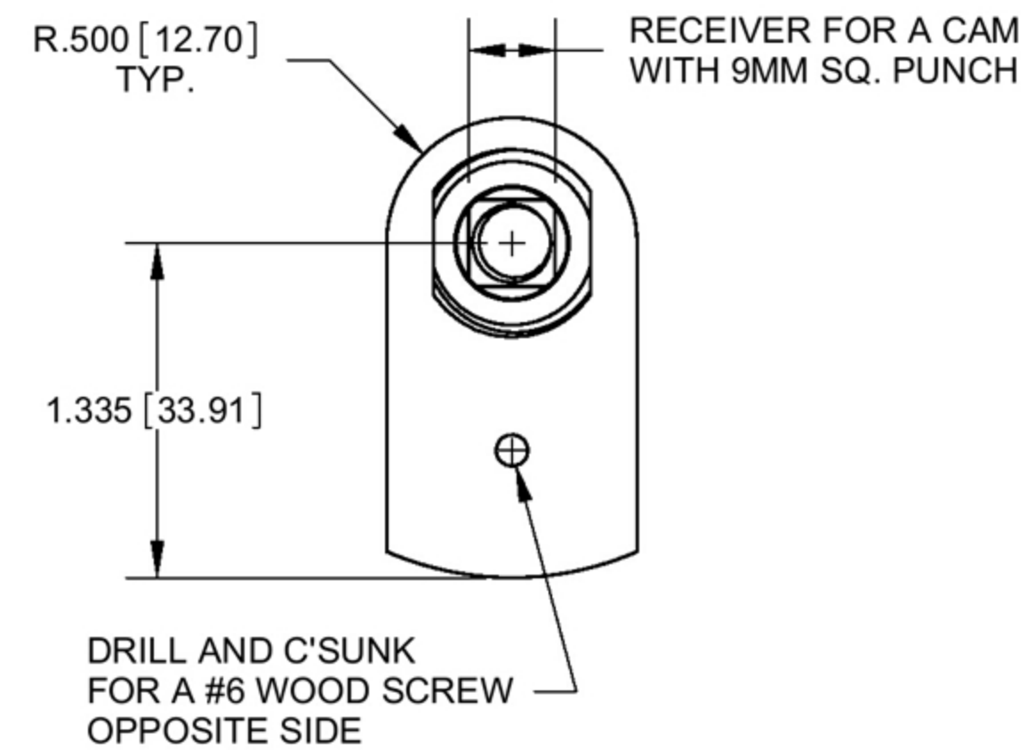
REAR VIEW
