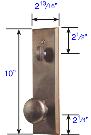
Standard interior trim Part # 451411/451512/451613
